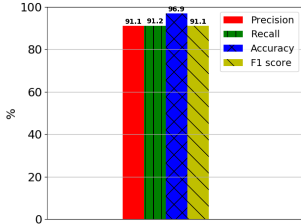
Figure 5.10: Optimized MVPS CNN classifier results
